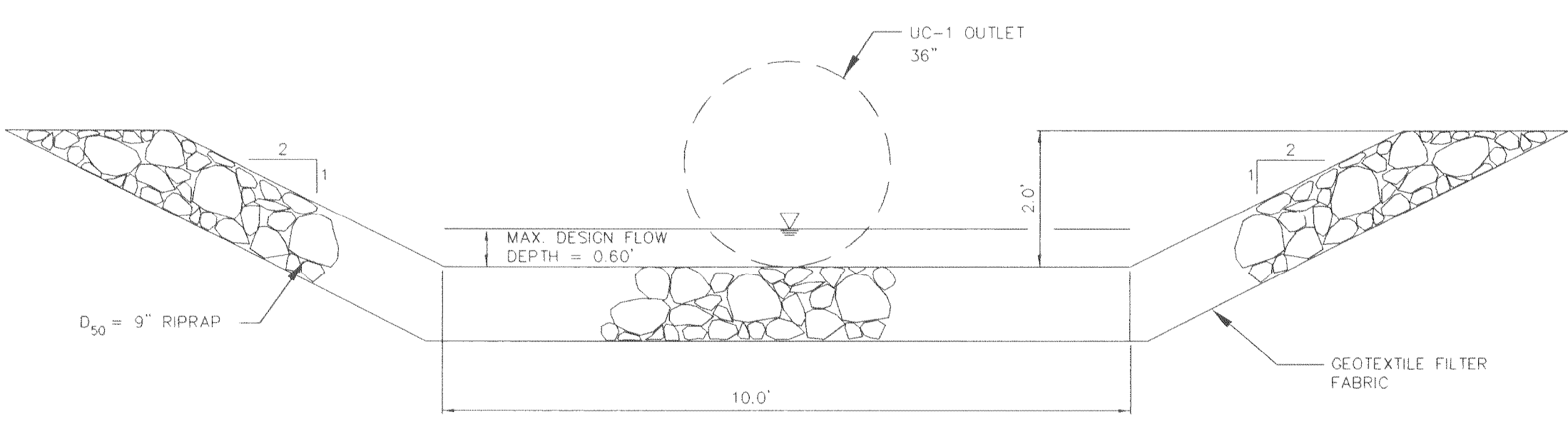
CROSS SECTION OF UC-1 OUTLET CHANNEL SCALE: 1" = 2'
