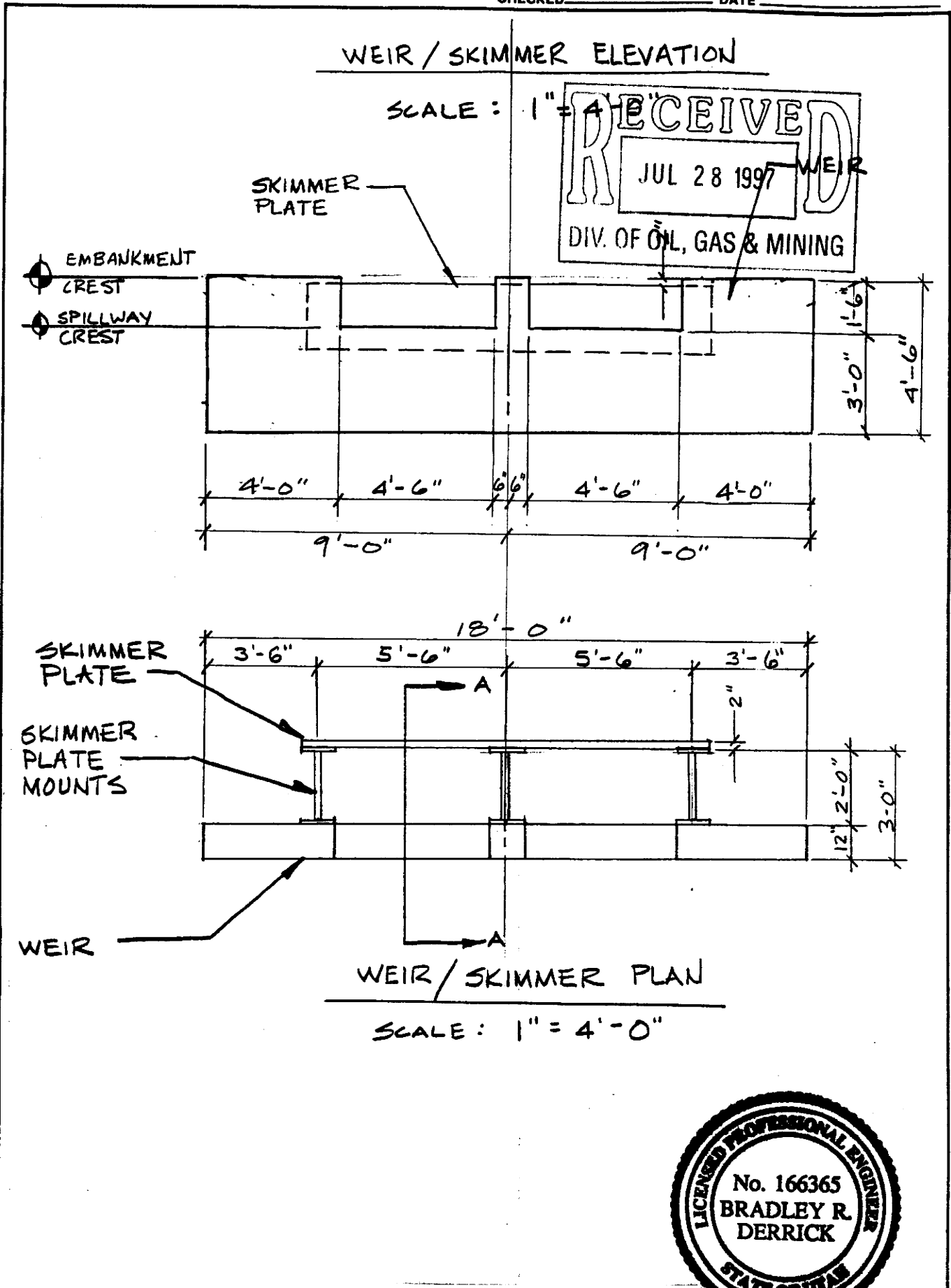
PLATE 7-6a. WEIR/OIL SKIMMER AND CROSS SECTION.
